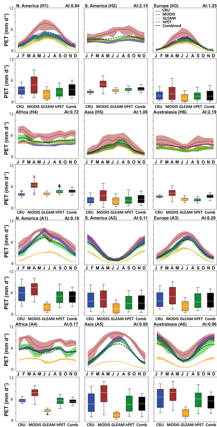
Fig. 4 Seasonal variations in PET for comparative datasets. Monthly distributions of PET for hPET and comparative datasets over the temporal domains listed in Table 2. Distributional medians are shown as white horizontal lines. Sample PET data, aggregated to common spatial ( 0.5^\circ ) and temporal (1 month) resolutions, separated according to humid versus arid locations on each study continent (N. America, S. America, Europe, Africa, Asia, Australasia), as shown in Fig. 2. We show comparisons for 2001–2018, corresponding to most of the temporal domain of MOD16 (note: some datasets were excluded from comparisons due to lack of data for relevant temporal domains). See caption for Fig. 3 for other relevant information.
