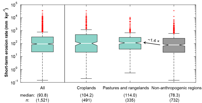
Figure 7. The comparison of global short-term erosion rates with and without anthropogenic influences. The extent of “croplands” and “pastures and rangelands” were digitised from Foley et al. (2005), and here it is shown that short-term erosion rates with anthropogenic influences are ~1.4 times higher than in non-anthropogenically impacted regions.
