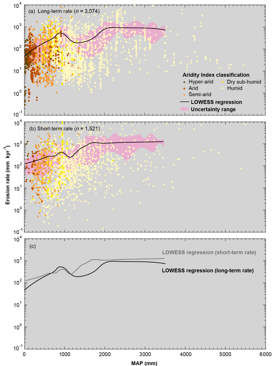
Figure 4. Relationships between mean annual precipitation (MAP) and (a) long-term erosion rates and (b) short-term erosion rates. Points are colour coded by Aridity Index categories. The black curve in each panel is the LOWESS regression, and the pink shading represents the uncertainty of the regression. (c) Comparison between LOWESS regressions between long- and short-term erosion rates. The regressions are truncated at extremely humid regions (MAP >3500 mm) owing to the limited number of data points in these regions.
