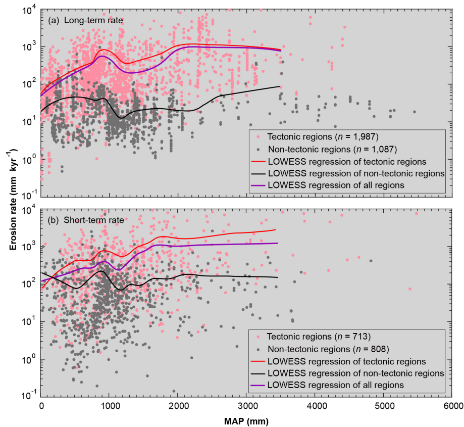
Figure 5. Relationships between mean annual precipitation (MAP) and long- (a) and short-term (b) erosion rates split into tectonic (pink) and non-tectonic (grey) regions. The red curve is the LOWESS regression for erosion versus MAP in tectonic regions, the black curve is the LOWESS regression for erosion versus MAP in non-tectonic regions, and the purple curve is the LOWESS regression for erosion versus MAP across all regions. The regressions are truncated at extremely humid regions (MAP > 3500 mm) owing to the limited number of data in these regions.
