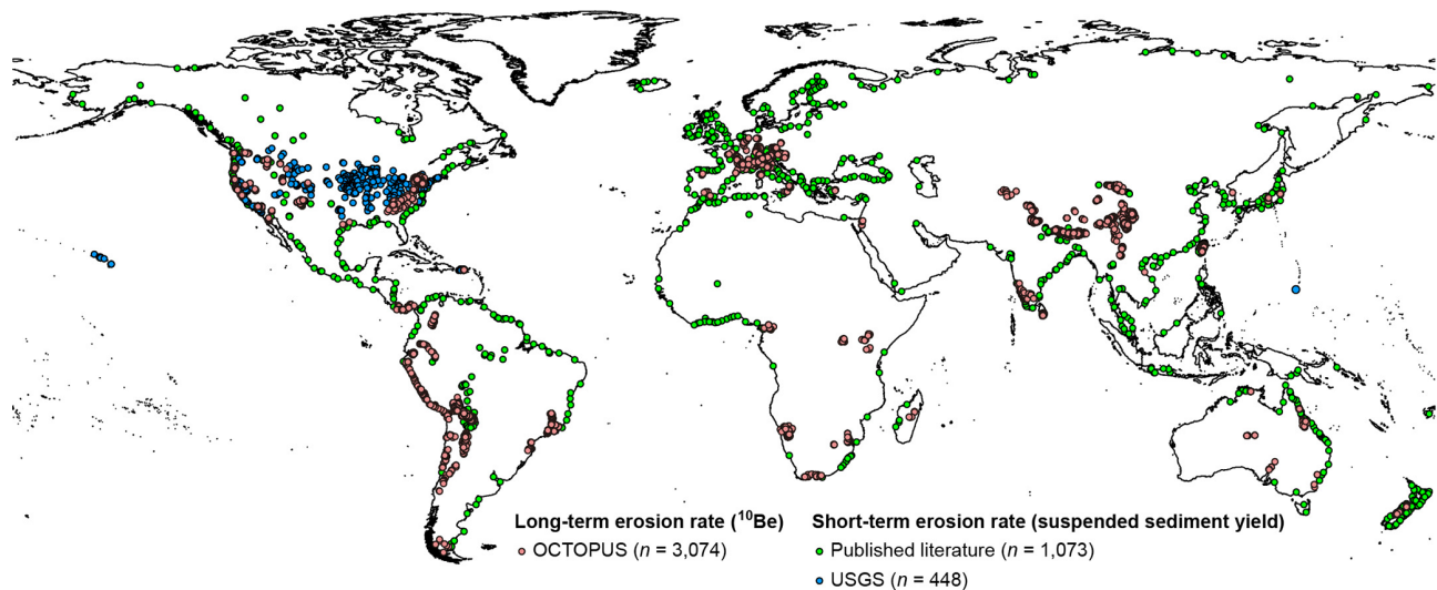
Figure 1. Global map of drainage basin erosion rate locations. Long-term erosion rates were obtained from OCTOPUS (Open Cosmogenic Isotope and Luminescence, red), estimated by ^{10}\text{Be} in the fluvial sediments. Short-term erosion rates were compiled from published literature (green) and USGS data (blue), determined by suspended sediment yield of gauging stations. The coastline is from Natural Earth ( https://www.naturalearthdata.com/ , last access: 19 May 2018) in the Pseudo Plate Carrée map projection.
