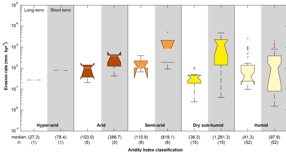
Figure 3. Long- and short-term erosion rates at co-located points as classified by the Aridity Index. Note that n = 79 is substantially smaller than the whole dataset (Fig. 2). However, the patterns evident in Fig. 2 are upheld in this limited co-located dataset.
