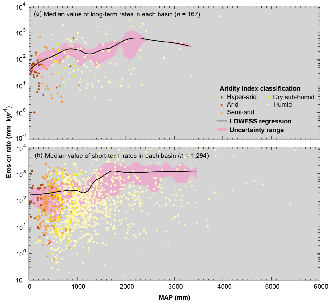
Figure A1. Relationships between mean annual precipitation (MAP) and (a) median value of long-term erosion rate in each basin and (b) median value of short-term erosion rate in each basin. Points are colour coded by Aridity Index categories. The black curve in each panel is LOWESS regression, and the pink shading represents the uncertainty of the regression. The regressions are truncated at extremely humid regions ( \text{MAP} > 3500 \text{ mm} ) owing to the limited number of data points in these regions.
