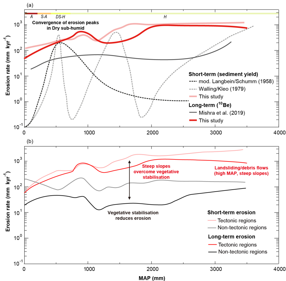
Figure 11. (a) Synthesis of non-linear relationships between MAP and short-term erosion rates (modified Langbein and Schumm, 1958 (see text), Walling and Kleo, 1979, and this study) and between MAP and long-term erosion rates (Mishra et al., 2019, and this study). (b) Relationships between short- and long-term erosion rates and MAP classified between tectonic and non-tectonic regions. MAP precipitation regimes akin to Aridity Index classes are shown along the top. The figure highlights the convergence of erosion peaks in Semi-arid and Dry sub-humid regions.
