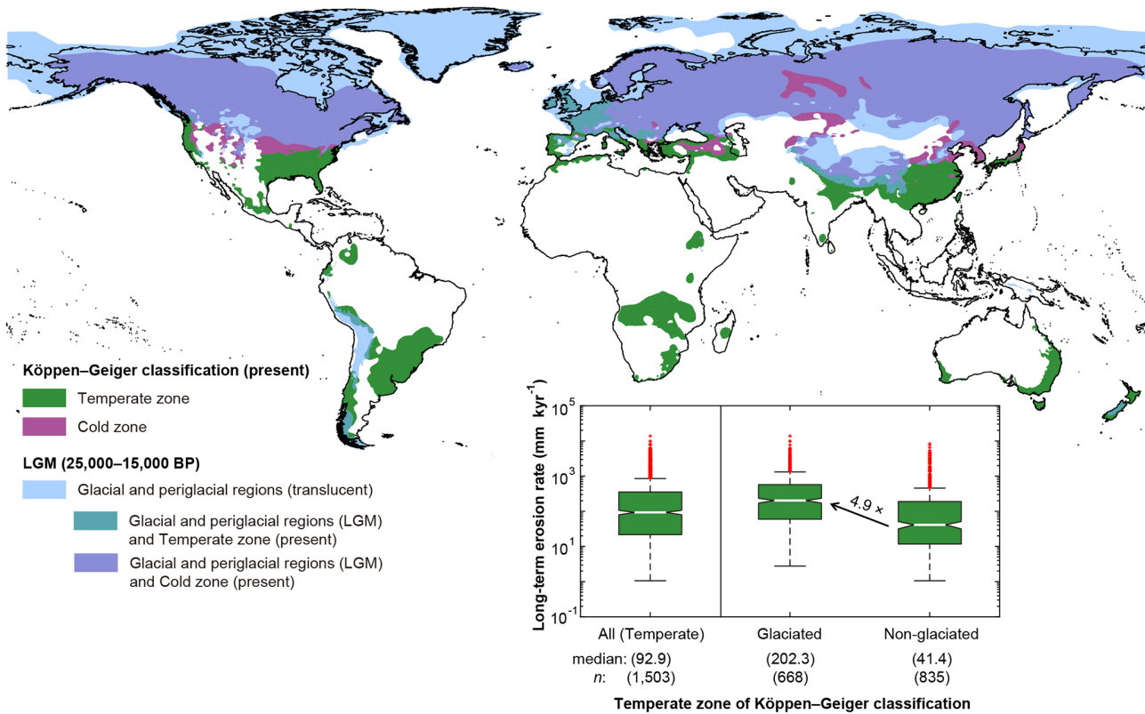
Figure 6. The extent of glacial and periglacial regions at the last glacial maximum (LGM) and the area of the Temperate and Cold zones of the Köppen–Geiger climate classification in the present. The glacial and periglacial regions were drawn from Ray and Adams (2001), according to the description in Sect. 3. The inset panel compares long-term erosion rates in the Temperate K–G zone with and without glacial influences at the LGM, indicating 4.9 times higher median erosion rates in formerly glaciated regions compared to non-glaciated regions.
